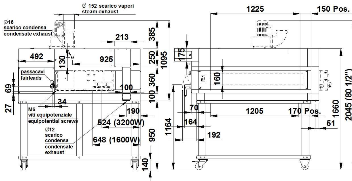
REAR VIEW
