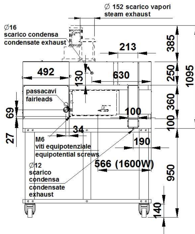
REAR VIEW
