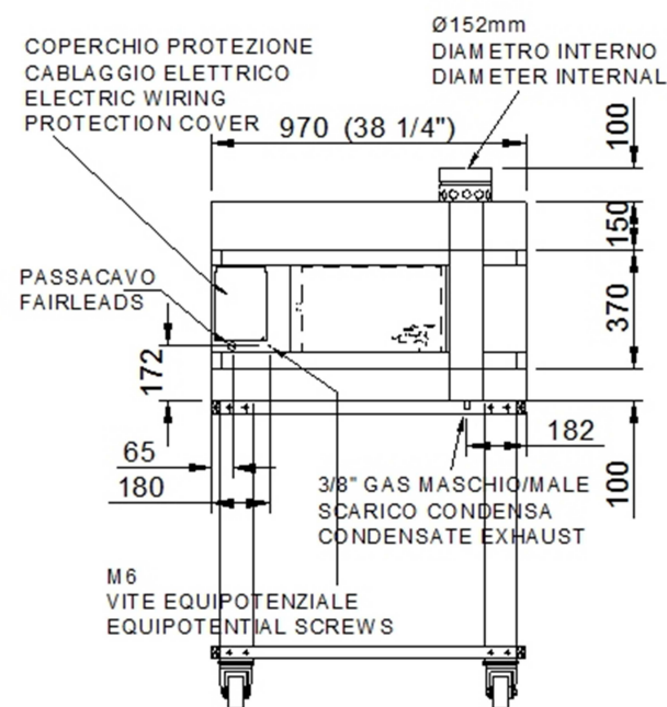
REAR VIEW
